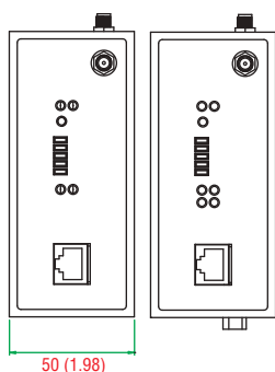
Front Views
